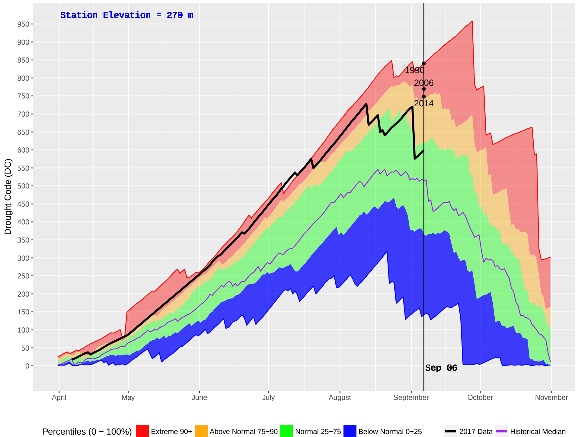
TALCHAKO (233) : Historical (1990–2016) and Current (2017) Noon Drought Code (DC)
